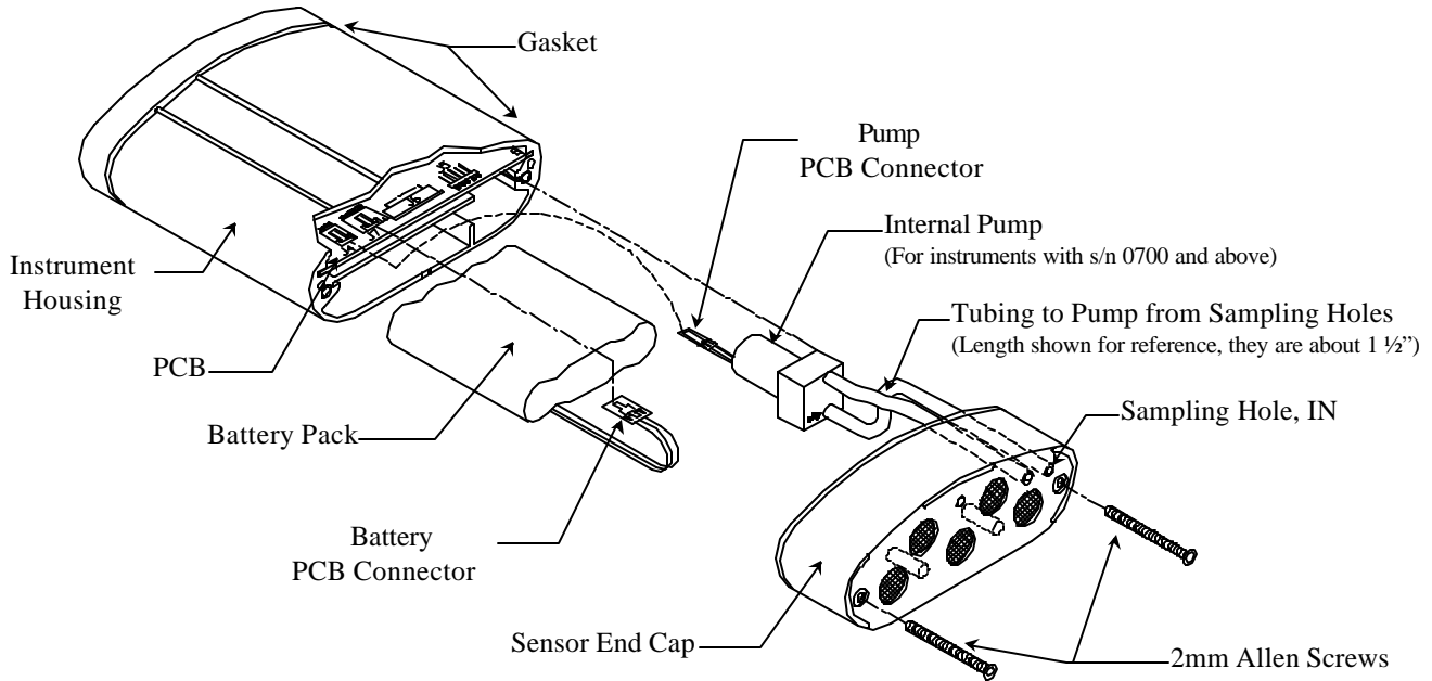
Figure 9: Replacing Battery Pack and Internal Pump
