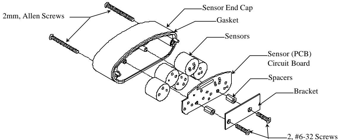
Figure 11: Replacing Sensors
