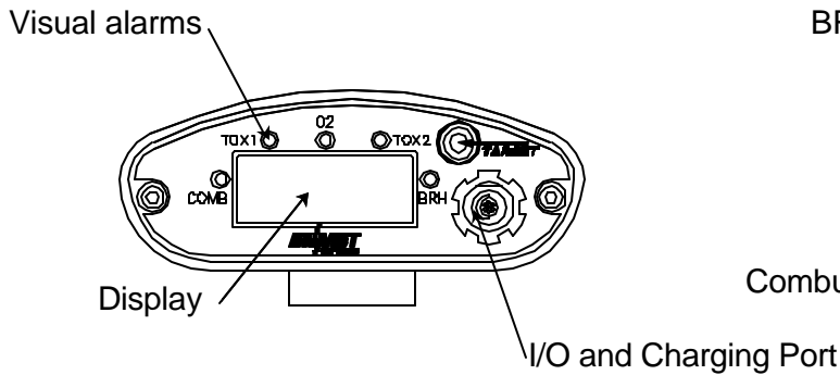
Figure 1: Front View
