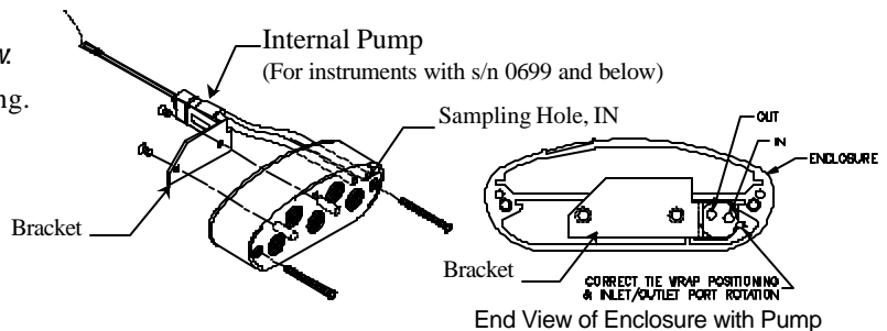
Figure 9a: Replacing Internal Pump for instruments with s/n 0699 and below
